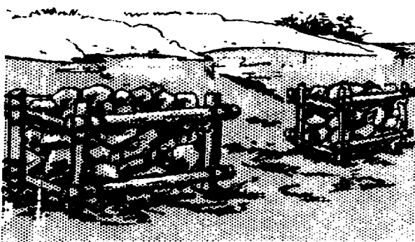
Figure 3-21. Rock-filled cribs.
